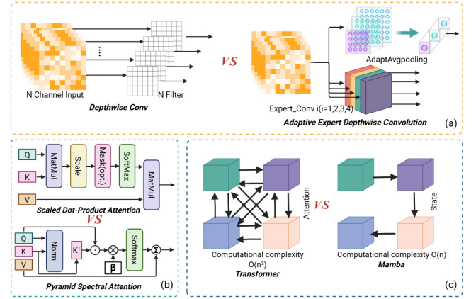
Fig. 1. Comparative analysis of innovation proposed in this study. (a) Depthwise versus AEDC module. (b) Scaled attention versus PSA module. (c) Transformer versus Mamba.
